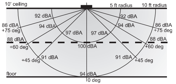
dBA measured in anechoic chamber 964/965 Series SPEAKER
