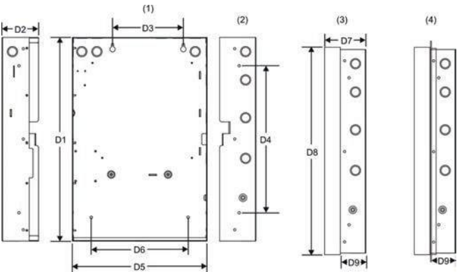
(1) Surface Mounting Holes (3) Backbox with Door Attached (2) Semi-flush Mounting Holes (4) Backbox with Door and Trim Kit attached
